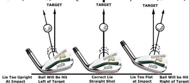
THE DIRECTIONAL IMPACT OF LIE ANGLES
